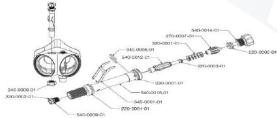
350M BIBS Mask Exhaust Regulator Assembly (540-0002-01)
