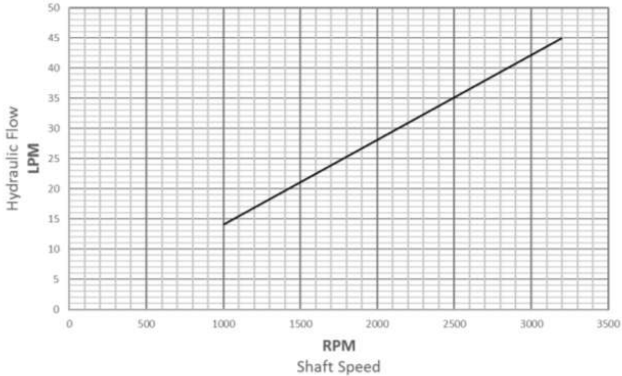
GR29 Hydraulic Flow Vs Shaft Speed
